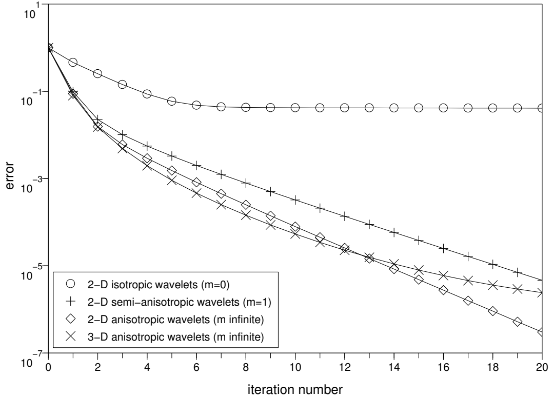
Figure 1: Convergence profiles of the wavelet Helmholtz algorithm with spline wavelets with different degrees of anisotropy
